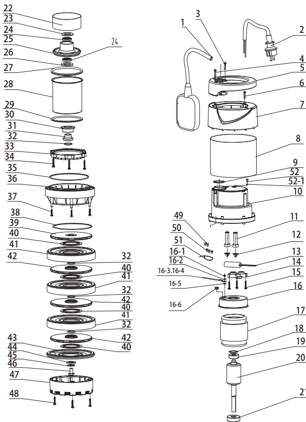
EXPLODED VIEW DRAWING - SPARE PARTS
